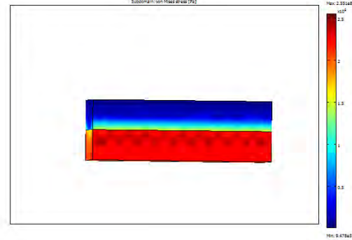
Figure 2. Stress Distribution in the Bimetallic Strip
