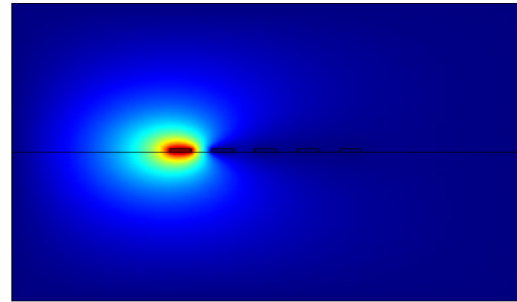
Figure 2. 2D surface potential distribution of five-conductor transmission lines, using port 1 as input.
