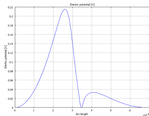
Figure 4. Potential distribution of five-conductor transmission lines interconnect in single layered dielectric region from (x,y) = (0,0) to (x,y) = (48,49) \mu m , using port 1 as input.
