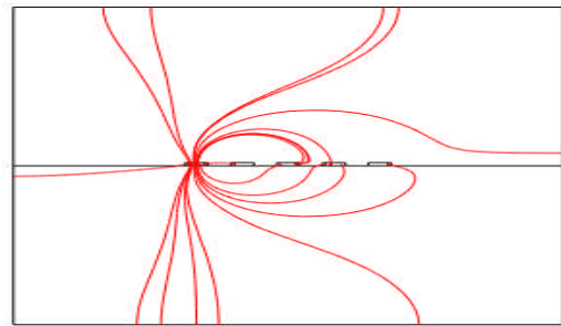
Figure 3. Streamline plot of five-conductor transmission lines interconnect in single layered dielectric region, using port 1 as input.
