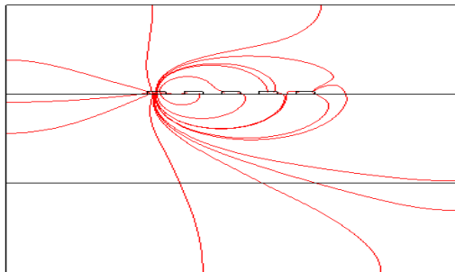
Figure 8. Streamline plot of five-transmission lines interconnect in two-layered dielectric media.
