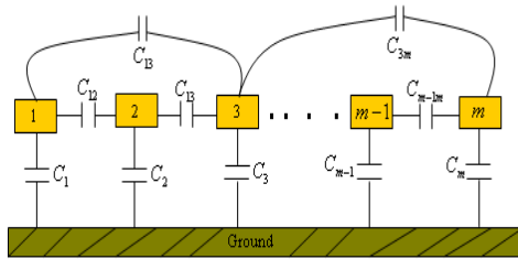
Figure 5. The per-unit length capacitances of a general m -conductor transmission line. For m -strip line, the per-unit-length capacitance matrix [C] is given by [13]
