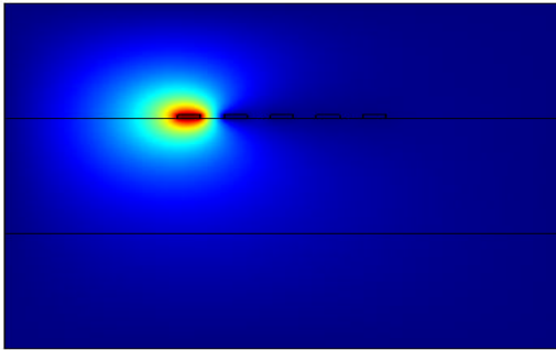
Figure 7. 2D surface potential distributions of five-transmission lines interconnect in two-layered dielectric media.
