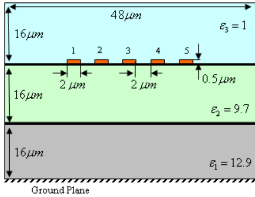
Figure 6. Cross-section of five-transmission lines interconnect in two-layered dielectric media.
