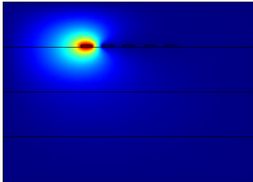
Figure 11. 2D surface potential distribution of five-transmission lines interconnect in three-layered dielectric media.
