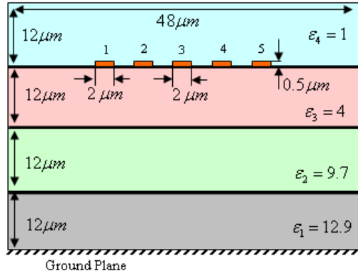
Figure 10. Cross-section of five-transmission lines interconnect in three-layered dielectric media.
