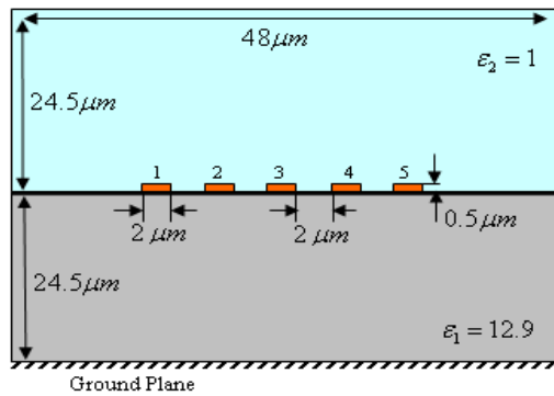
Figure 1. Cross-section of five-conductor transmission lines interconnect in single layered dielectric region.
