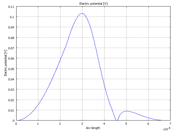
Figure 9. Potential distribution of five-transmission lines interconnect in two-layered dielectric media.
