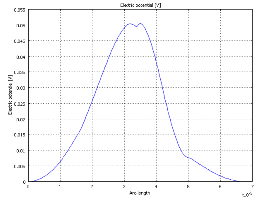
Figure 12. Potential distribution of five-transmission lines interconnect in three-layered dielectric media.
