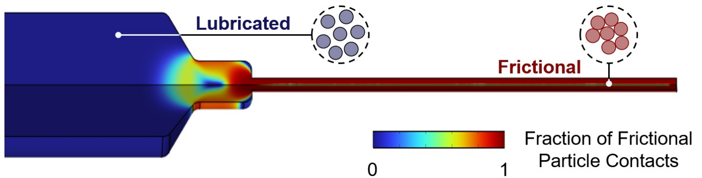
Figure 2 : CFD simulation of a particulate suspension through a syringe needle (particle volume fraction of 50%, particle diameter of 10 \mu m ). Contours show transition from lubricated to frictional particle contacts, which leads to shear thickening and clogging.
