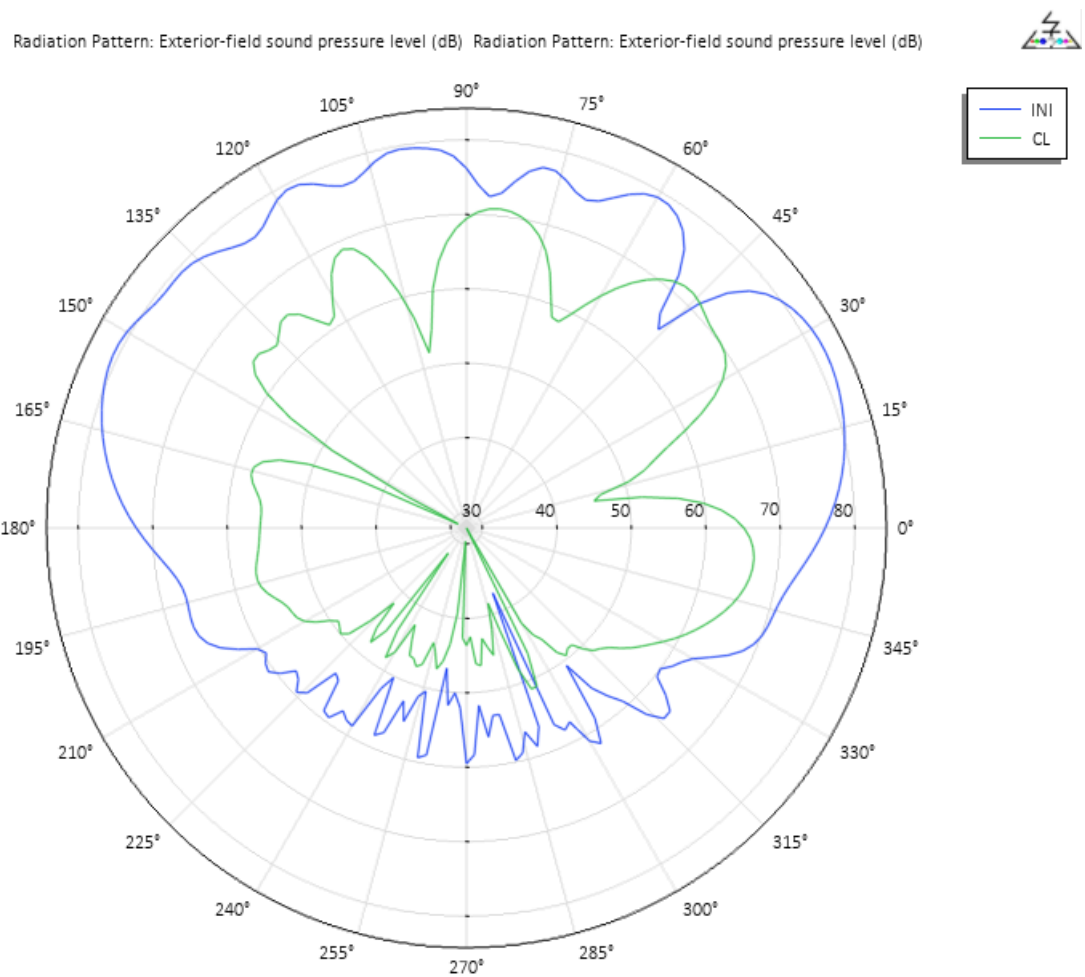
Figure 4 : Radiation Pattern of exterior-field sound pressure level (dB) of with and without cloak.
