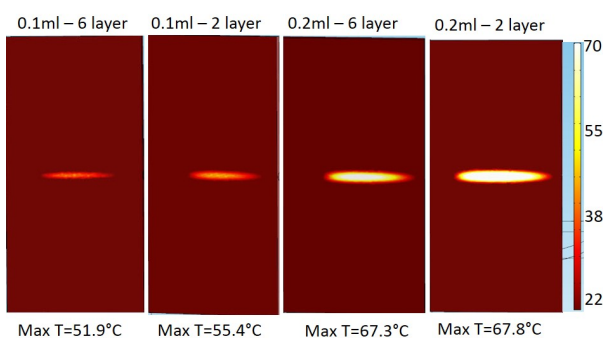
Figure 1 : Simulation of thermal signal on surface of Kevlar/epoxy matrix composite specimen;
