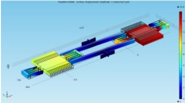
Figure 1 : Mechanically Coupled Resonators Displacement Graph at loaded sides resonant frequency.
