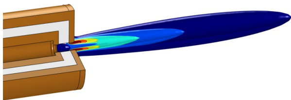
Figure 1 : Figure 1: Temperature distribution associated with micro plasma jet
