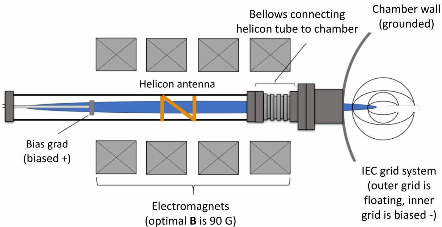
Figure 1 : HIIPER Schematic
