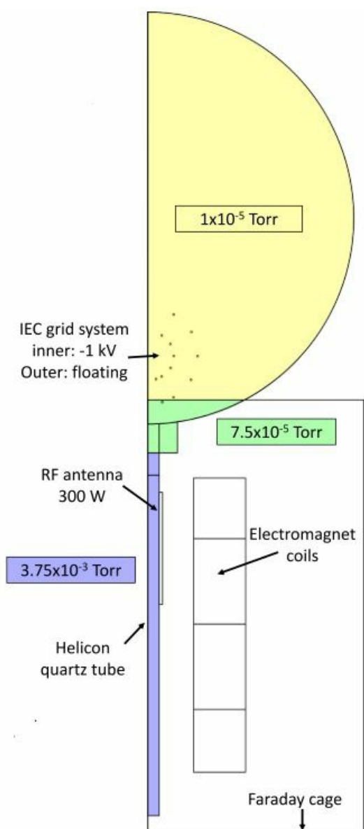
Figure 1 : HIIPER Schematic
