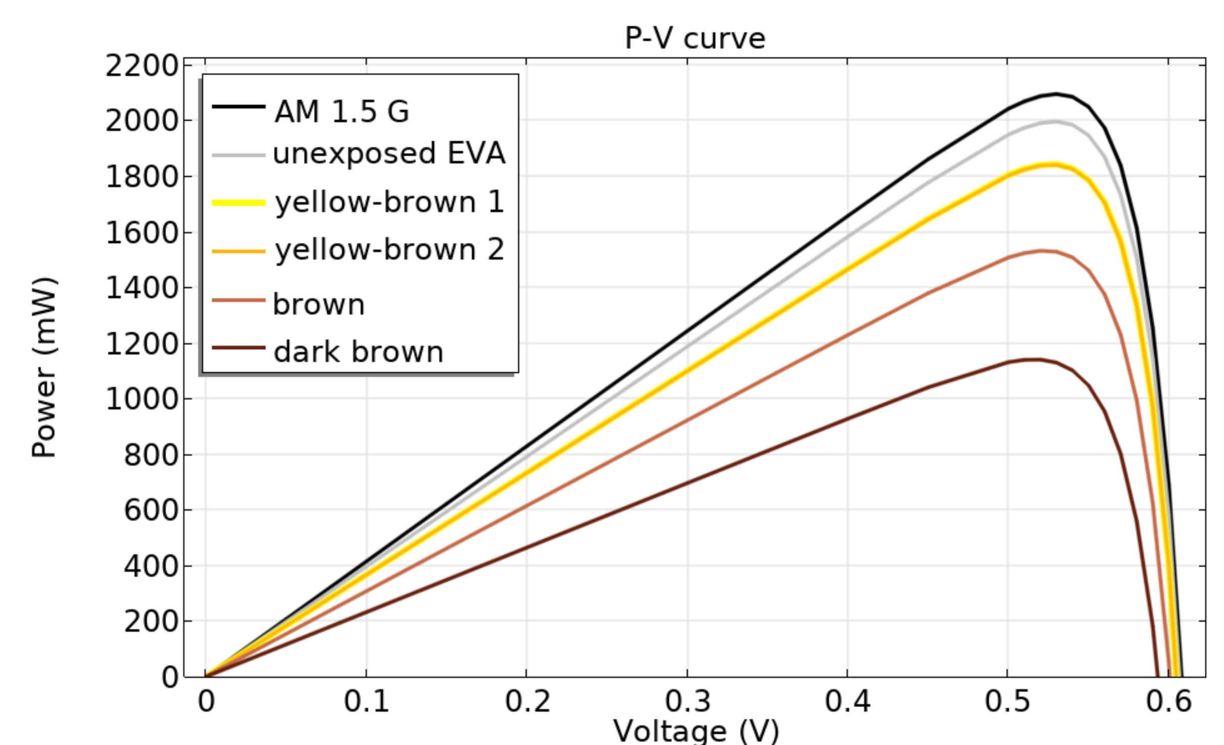
Figure 3. P-V curve of the solar cell at different levels of yellowing.
