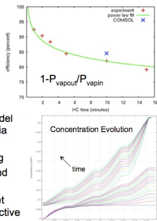
Figure 3: IBD model and results.
