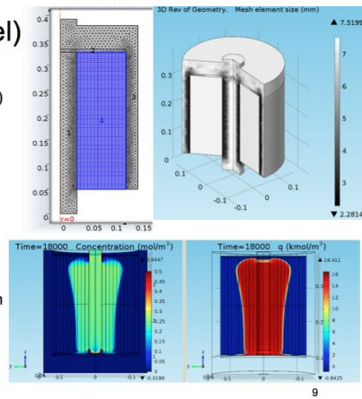
Figure 4: Microlith model and simulation results.
