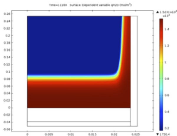
Figure 1: Concentration gradient in 2-D axisymmetric simulation of adsorption in a fixed bed.
