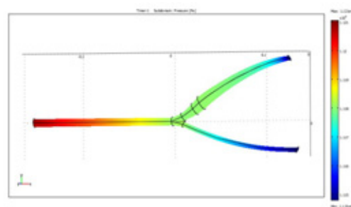
Figure 7 Pressure Field
